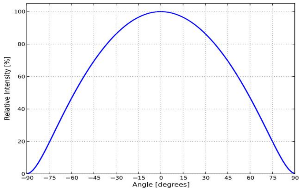
Typical radiation pattern for T at test current, T_j = 25^{\circ}\text{C} .
