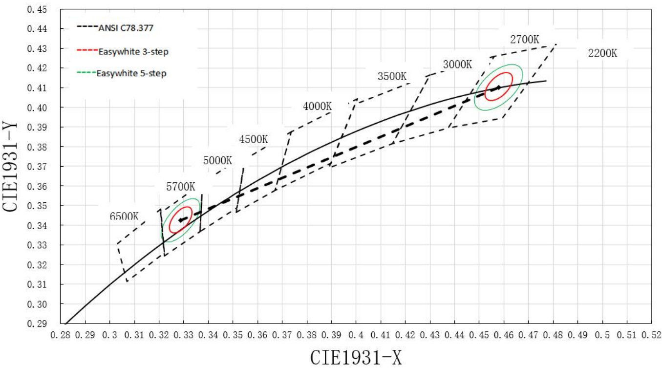
CIE(X,Y)坐标 CIE coordinates (X, Y)
