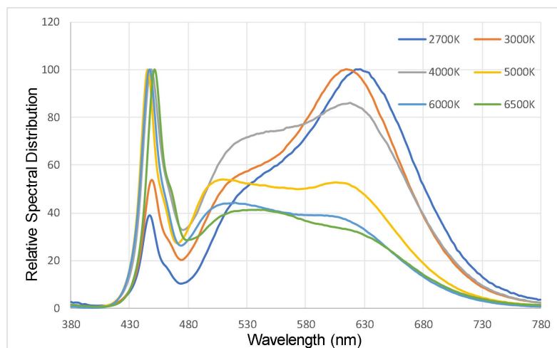
Figure 1a. Typical normalized power vs. wavelength for at test current, RA90 Tj=25°C.
