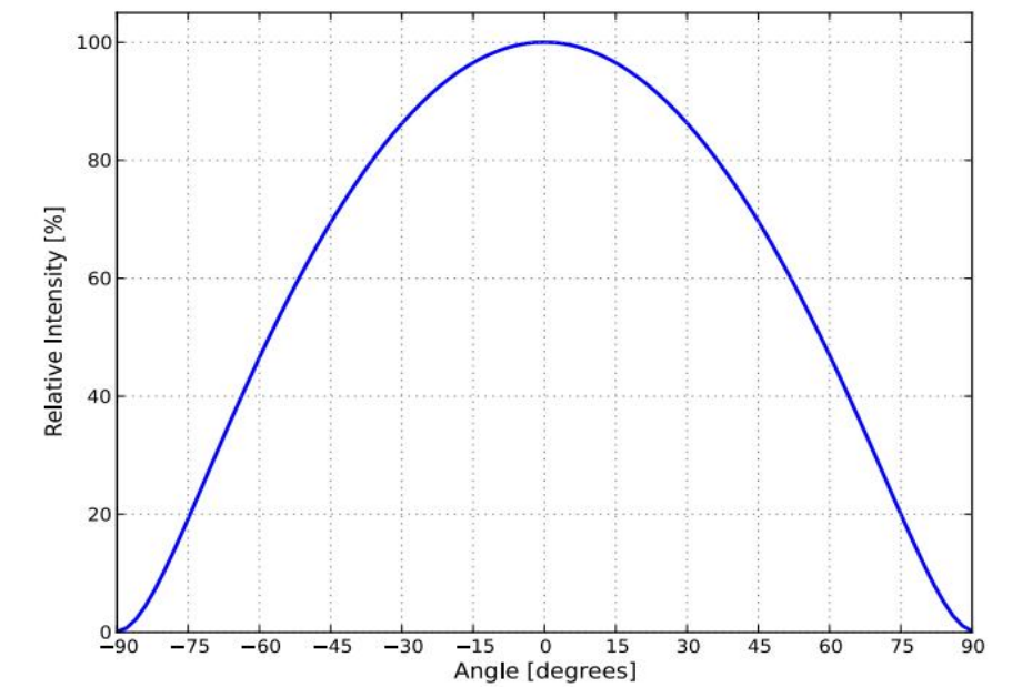
Typical radiation pattern for T at test current, Tj=25°C.
