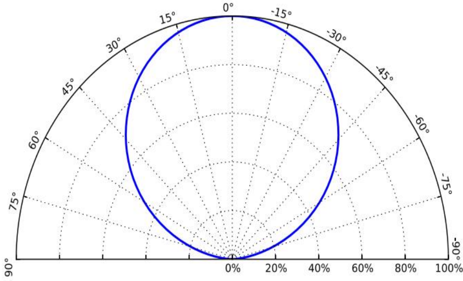
Typical radiation pattern for T at test current, Tj =25℃.
