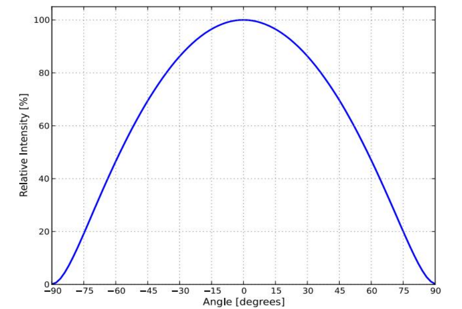
Typical radiation pattern for T at test current, T_j=25^{\circ}\text{C} .
