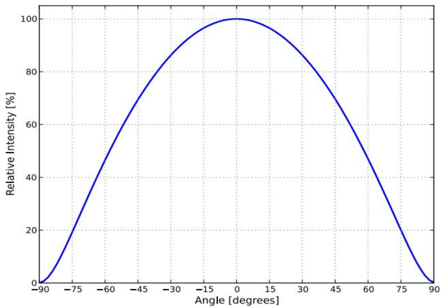
Typical radiation pattern for T at test current, T_j=25^{\circ}\text{C} .
