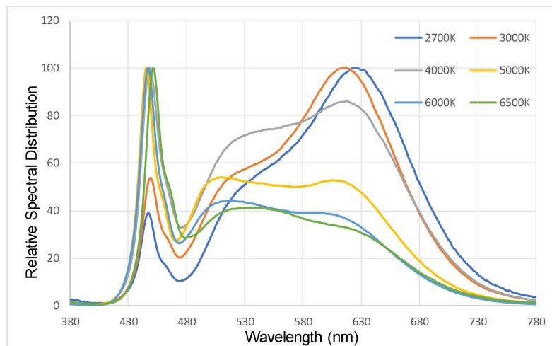
Figure 1a. Typical normalized power vs. wavelength for at test current, RA90 T_j = 25^\circ \text{C} .
