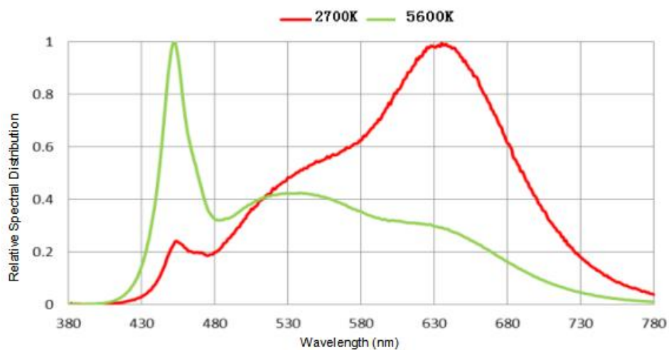
Figure 1a. Typical normalized power vs. wavelength for at test current, RA95 T_j = 25^\circ \text{C} .
