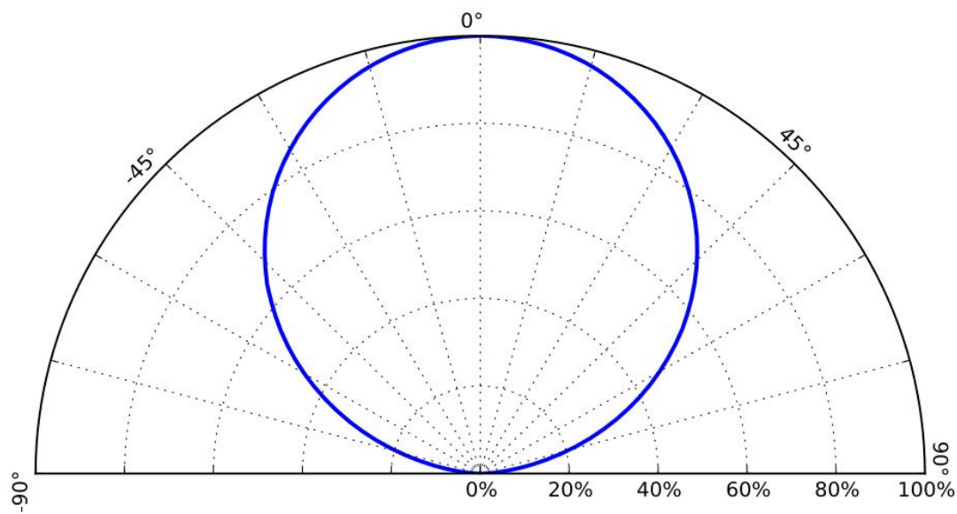
Typical radiation pattern for T at test current, Tj =25° C.
