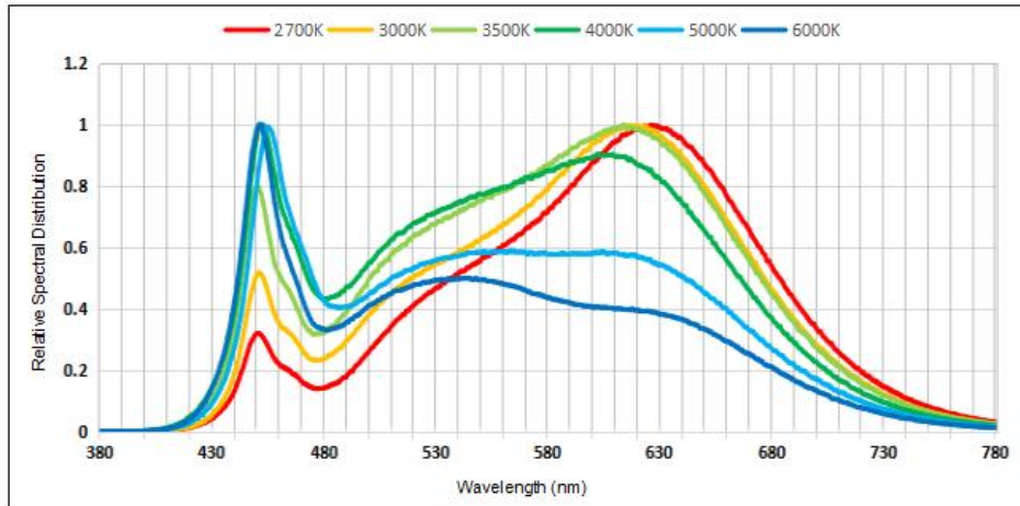
Figure 1a. Typical normalized power vs. wavelength for at test current, RA90 T_j = 25^\circ \text{C} .
