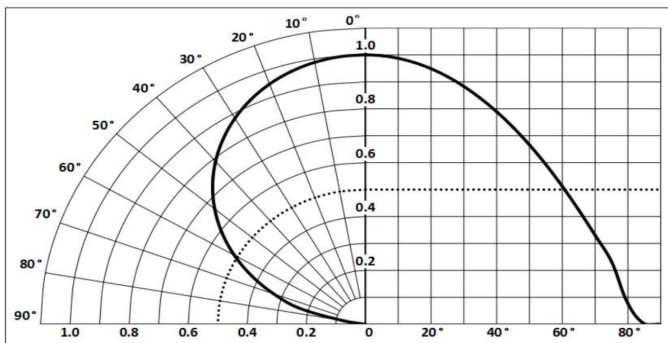
Radiation Pattern Characteristics ( T_j=25^{\circ}\text{C}/I_F=700\text{mA} )
