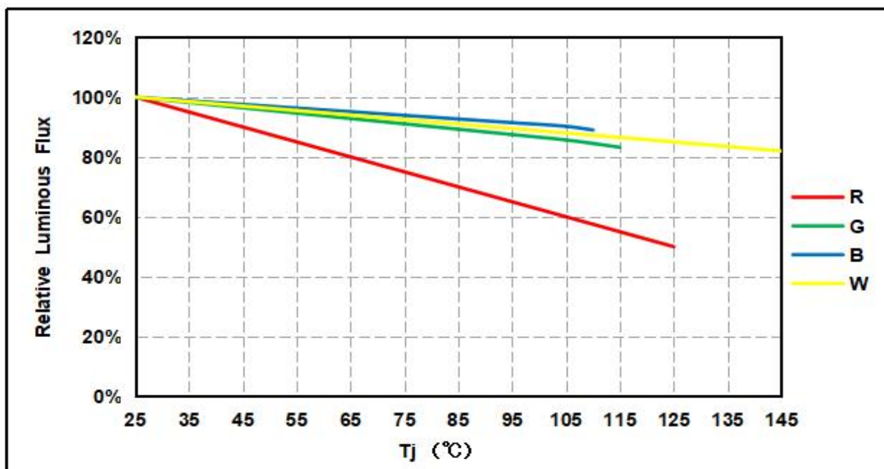
Relative Luminous Intensity VS Junction Temperature ( I_F=350\text{mA} , 25^\circ\text{C} )
