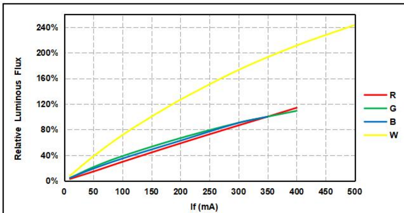
Relative Luminous Flux VS Forward Current ( I_F=350\text{mA} , 25^\circ\text{C} )
