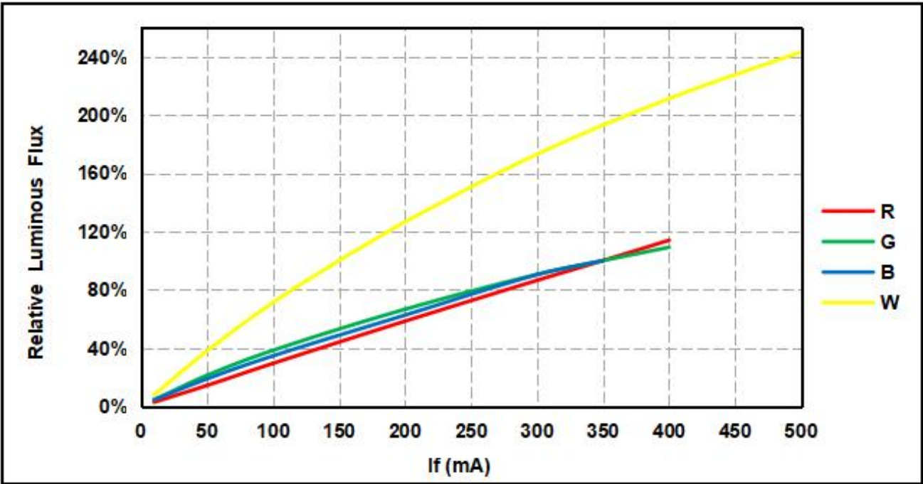
Relative Luminous Flux VS Forward Current (IF=350mA, 25°C)
