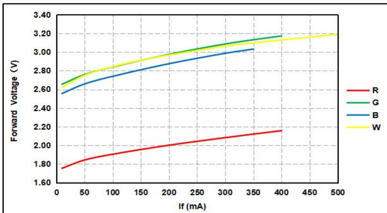
Forward Voltage VS Forward Current ( I_F=350\text{mA} , 25^\circ\text{C} )
