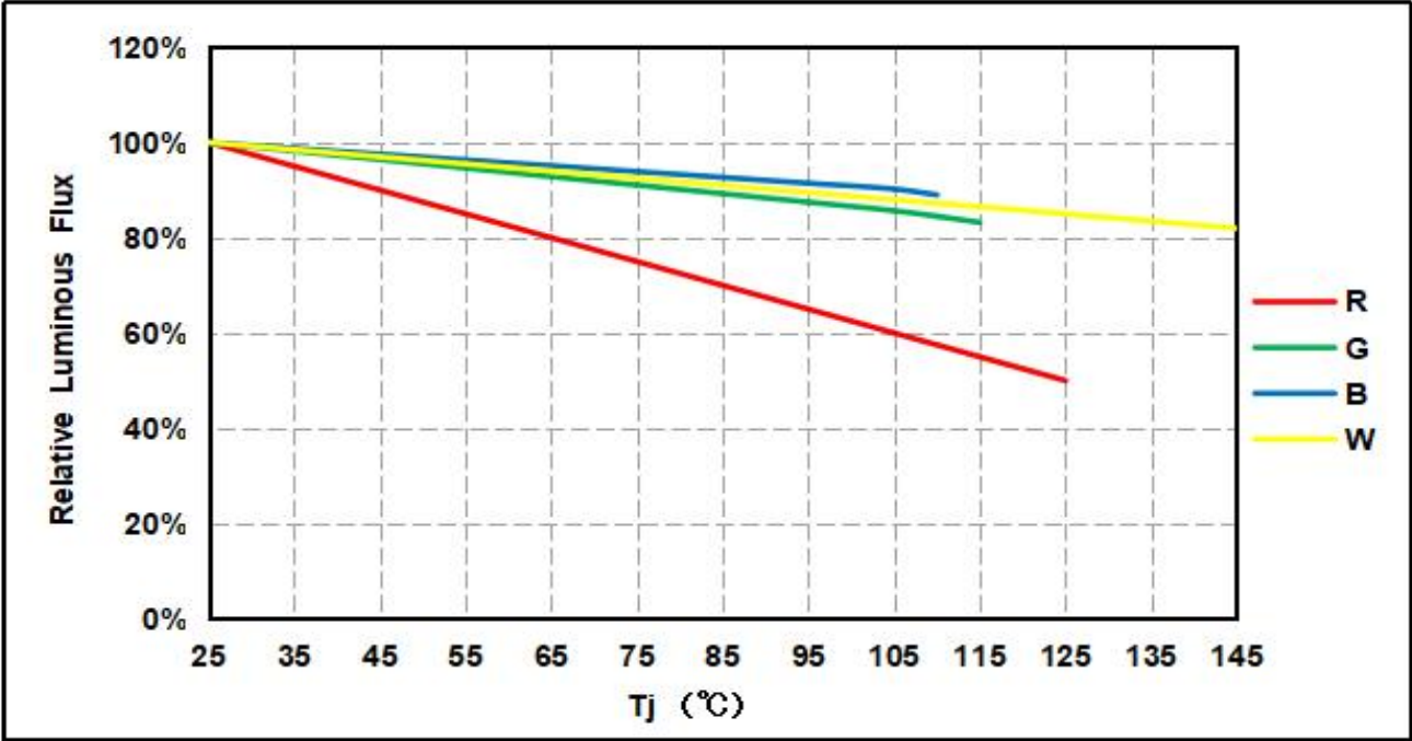
Relative Luminous Intensity VS Junction Temperature (IF=350mA, 25°C)
