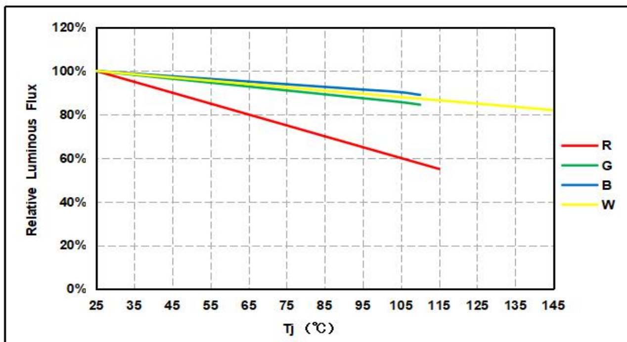
Relative Luminous Flux VS Junction Temperature ( I_F=150\text{mA} , 25^\circ\text{C} )
