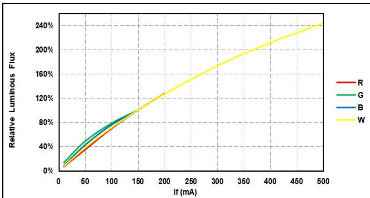
Relative Luminous Flux VS Forward Current ( I_F=150\text{mA} , 25^\circ\text{C} )
