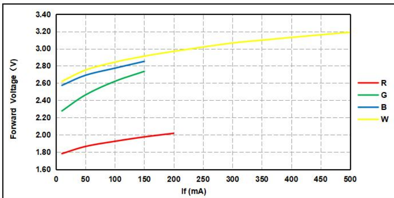
Forward Voltage VS Forward Current ( I_F=150\text{mA} , 25^\circ\text{C} )
