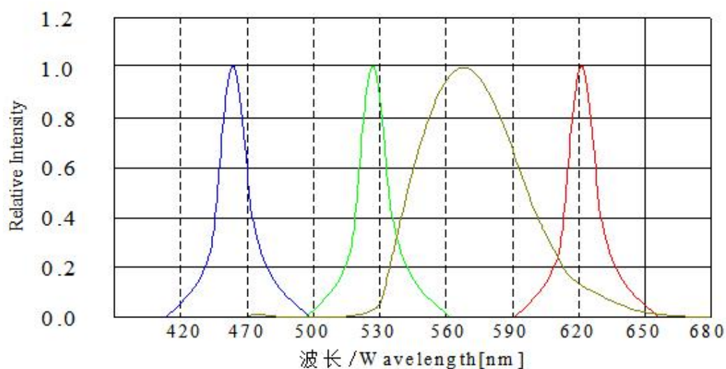
Figure 1a. Typical normalized power vs. wavelength for at test current, RA80 Tj =25° C.
