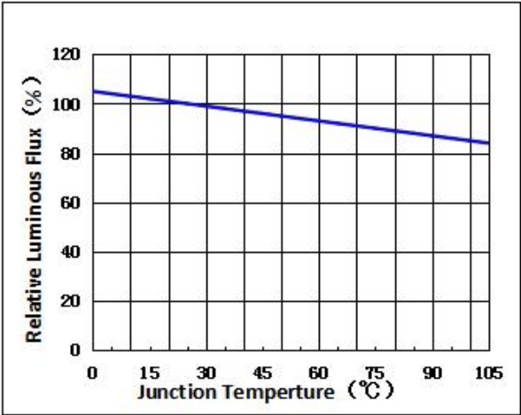
Relative Luminous Intensity VS Junction Temperature.
