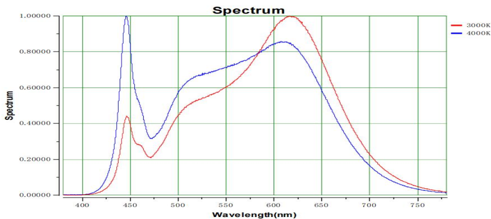
Figure 1a. Typical normalized power vs. wavelength for at test current, RA90 Tj =25° C.
