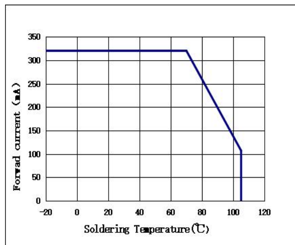
Forward Current VS Soldering Temperature.
