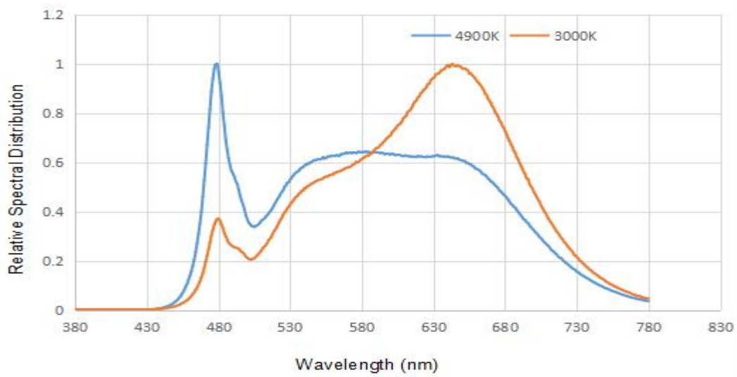
Figure 1a. Typical normalized power vs. wavelength for at test current, RA90 T_j = 25^\circ \text{C} .
