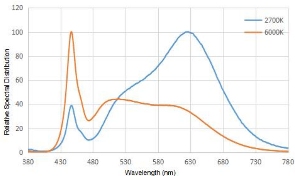
Figure 1a. Typical normalized power vs. wavelength for at test current, RA90 Tj =25° C.
