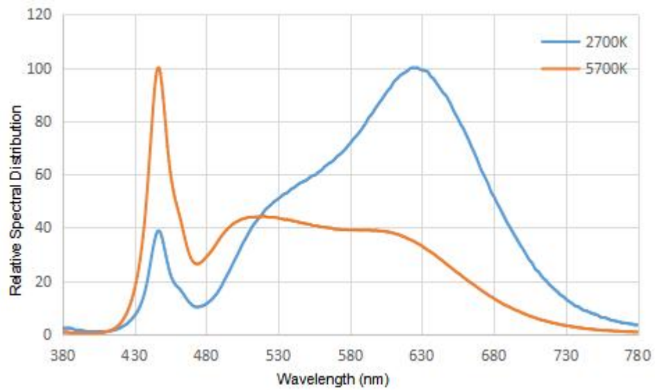
Figure 1a. Typical normalized power vs. wavelength for at test current, RA70 Tj =25° C.
