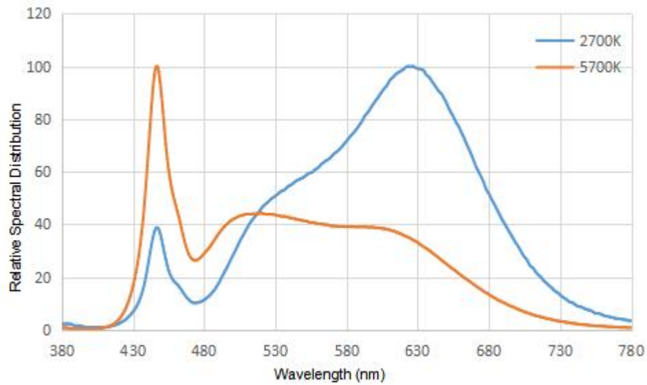
Figure 1a. Typical normalized power vs. wavelength for at test current, RA95 Tj =25° C.
