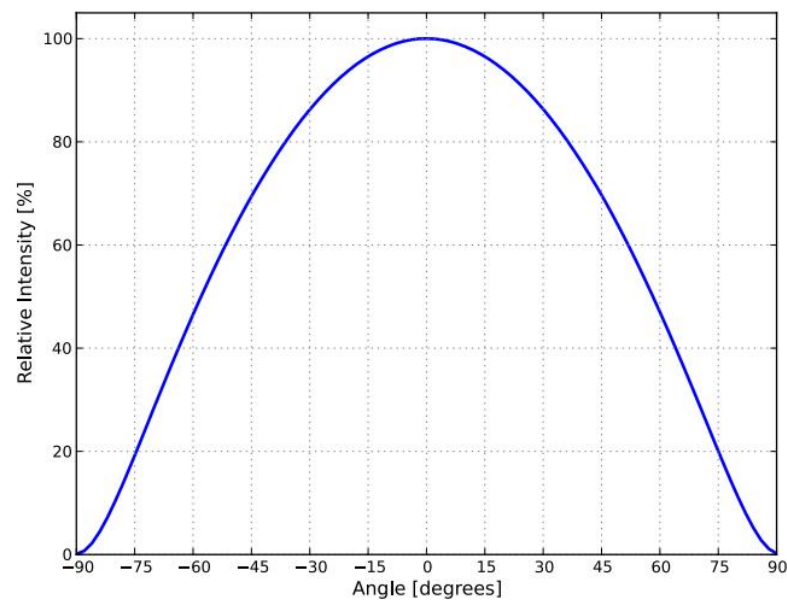
Typical radiation pattern for T at test current, T_j = 25^{\circ}\text{C} .
