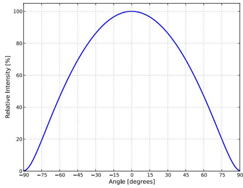
Typical radiation pattern for T at test current, Tj =25° C.
