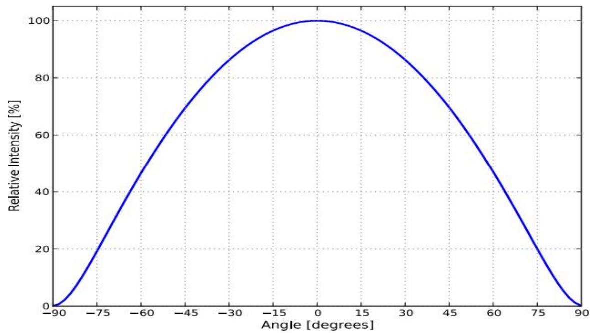
Typical radiation pattern for T at test current, Tj =25° C.
