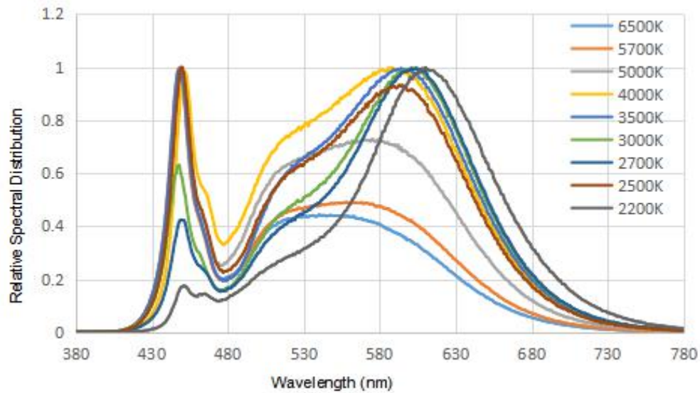
Figure 1a. Typical normalized power vs. wavelength for at test current, RA80 T_j = 25^\circ \text{C} .
